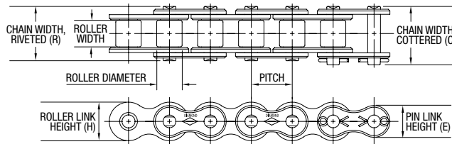
Single Strand
