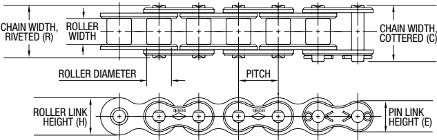
Single Strand
