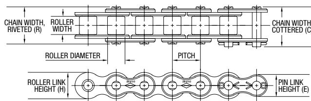
Standard Chain
