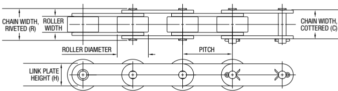
Oversized Roller Conveyor Series (C2XX2)
