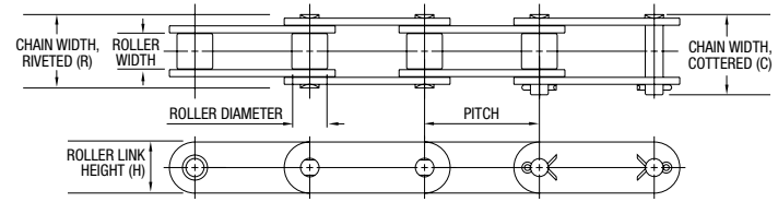
Conveyor Chain (C20X0)
