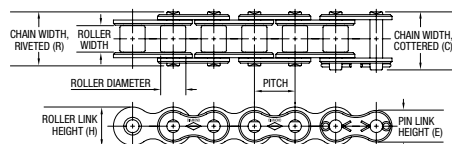
Single Strand
