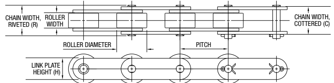
Oversized Roller (C2XX2)
