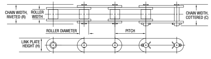
Oval contour (C20X0)
