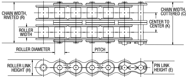
Multistrand Chain (-X Suffix)
