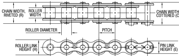
Standard Chain
