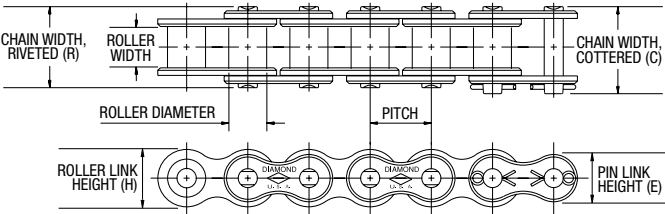
Standard Chain
