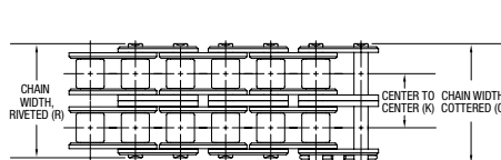
Multiple Strand (-X suffix)
